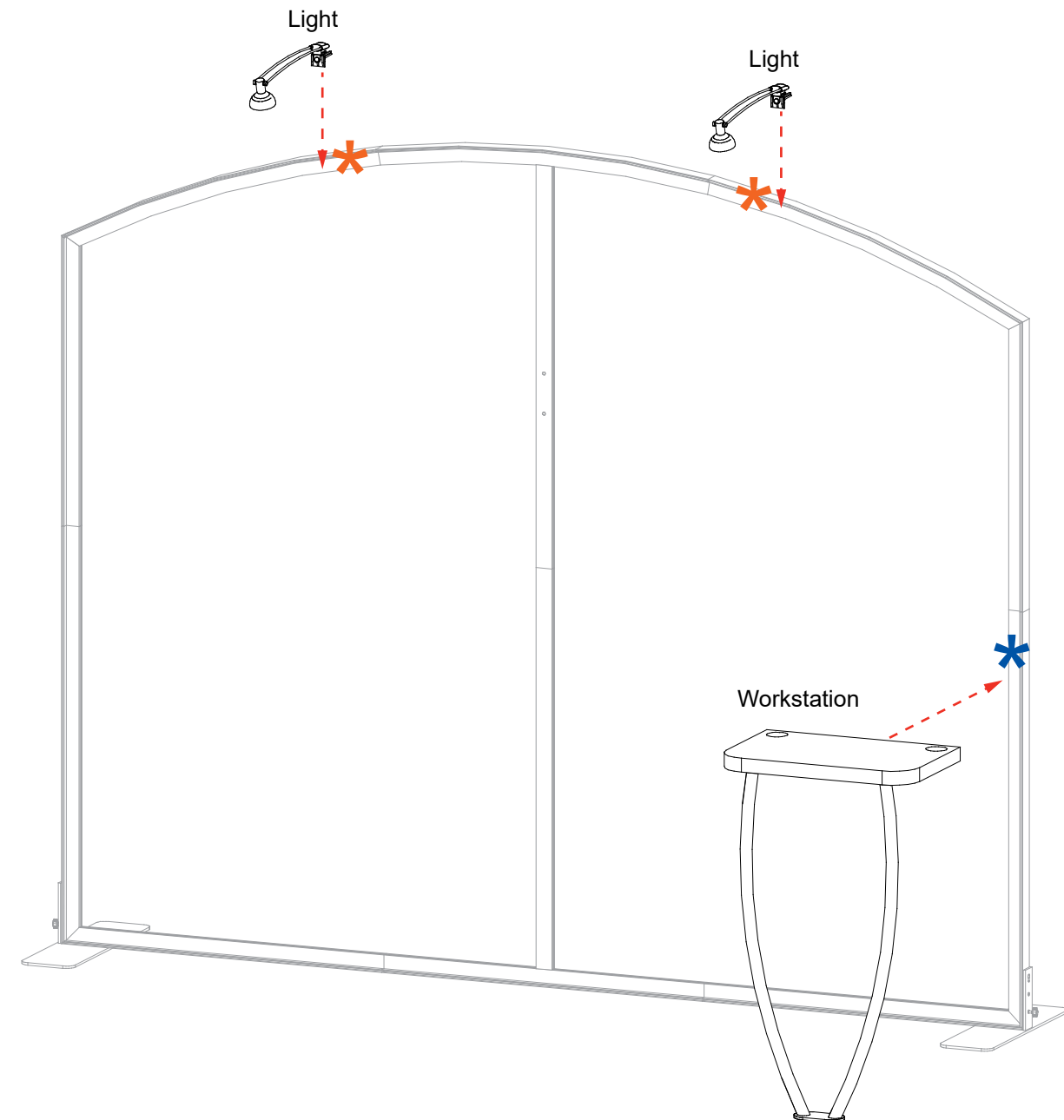
Completed Assembly
